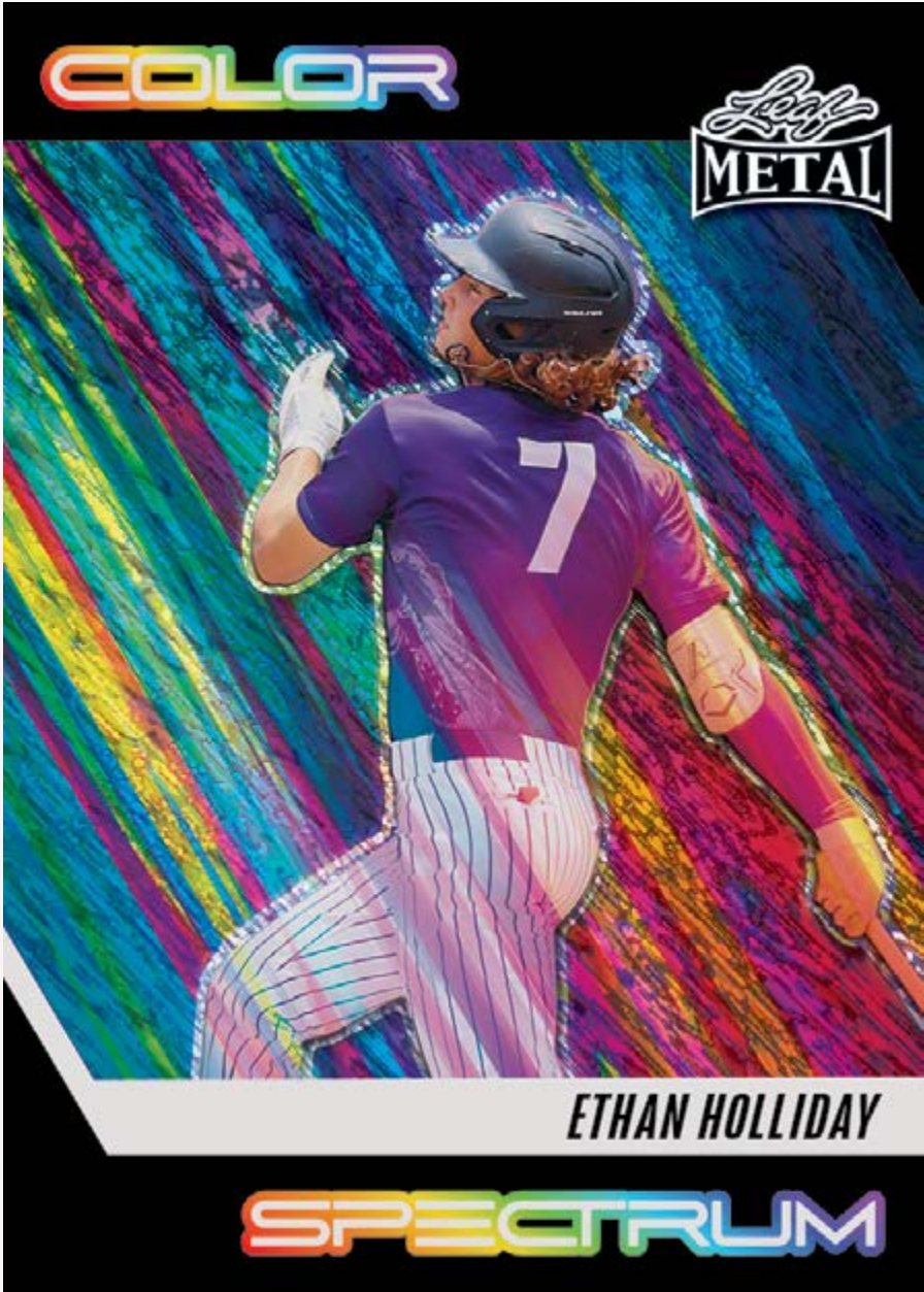
COLOR SPECTRUM
